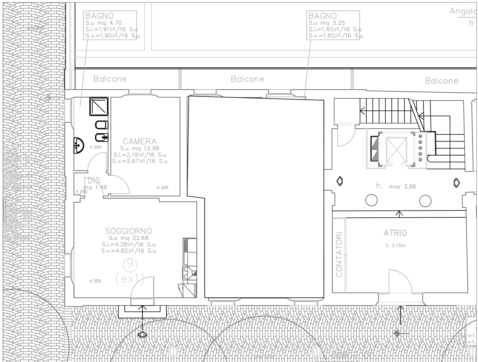
Via Alessandrini 21 (BO) PT INT. 9 (scala 1:100)
